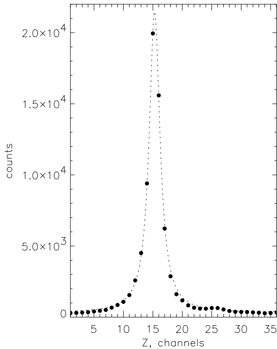
Figure 8: An example of the spectrum of the calibration line HeIX6678 scanned with the interferometer Fp500 (dots) and its fitting by the Lorentz profile.
